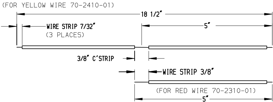
WIRE DETAIL "B"
