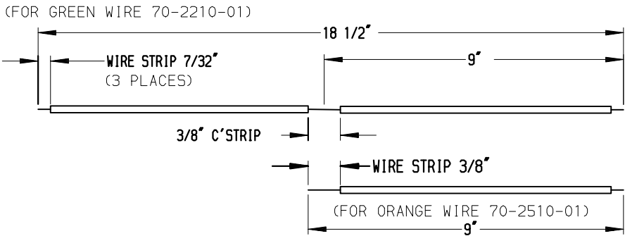
WIRE DETAIL "A"
